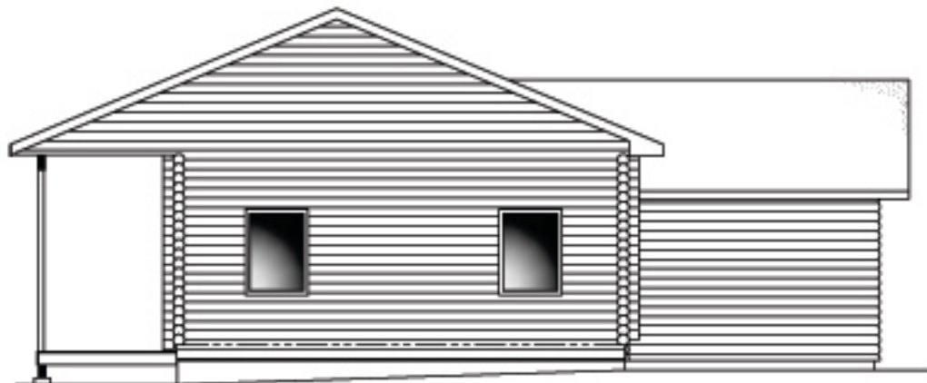
THE CEDAR RIDGE - RIGHT SIDE ELEVATION
