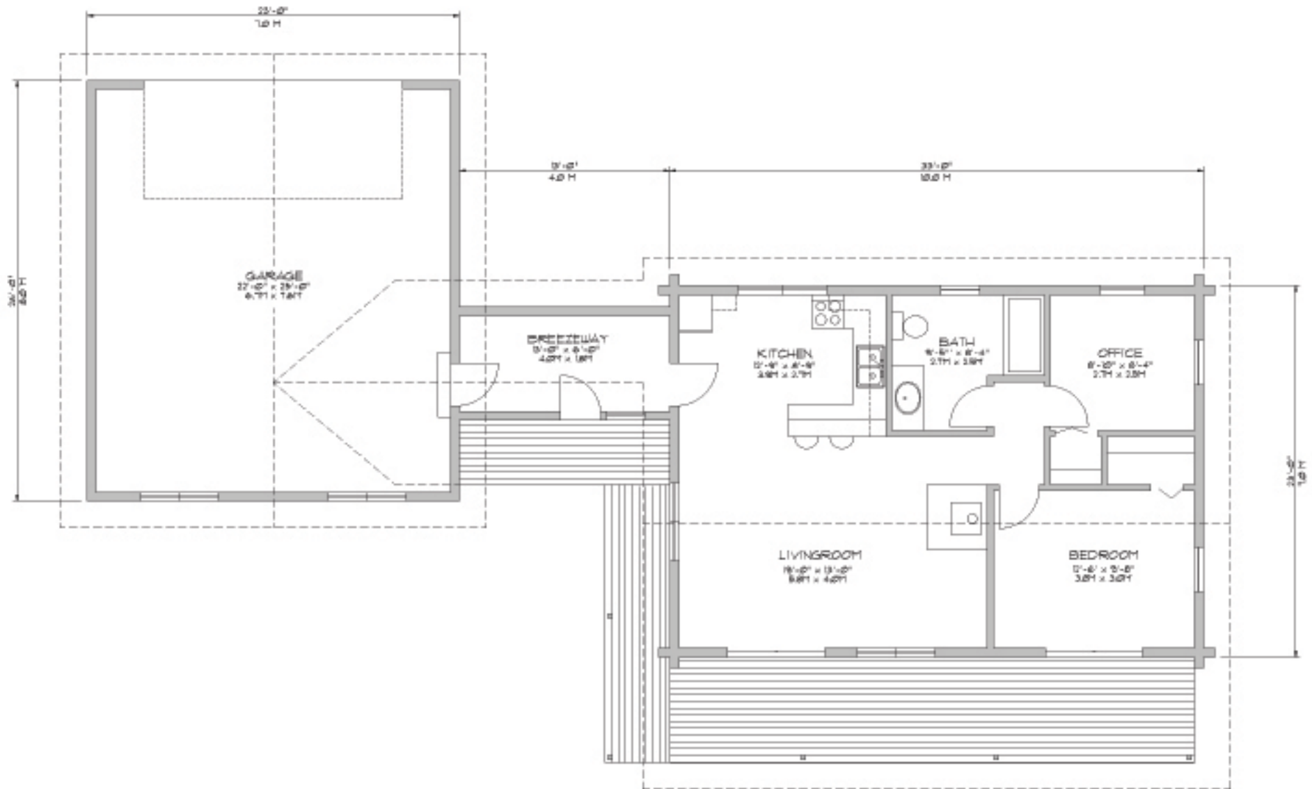
THE CEDAR RIDGE - MAIN FLOOR PLAN
