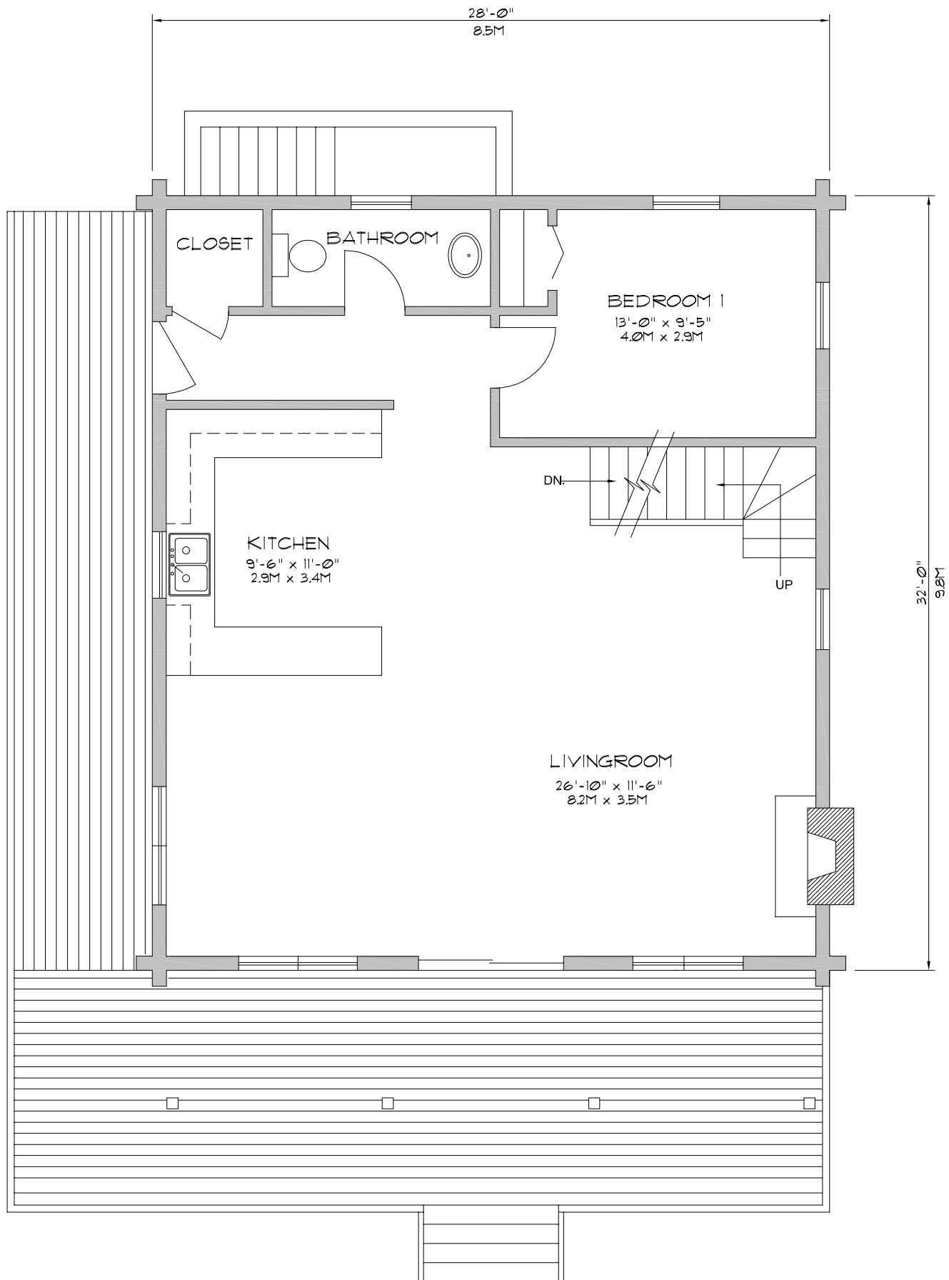
THE CHALET - MAIN FLOOR PLAN
