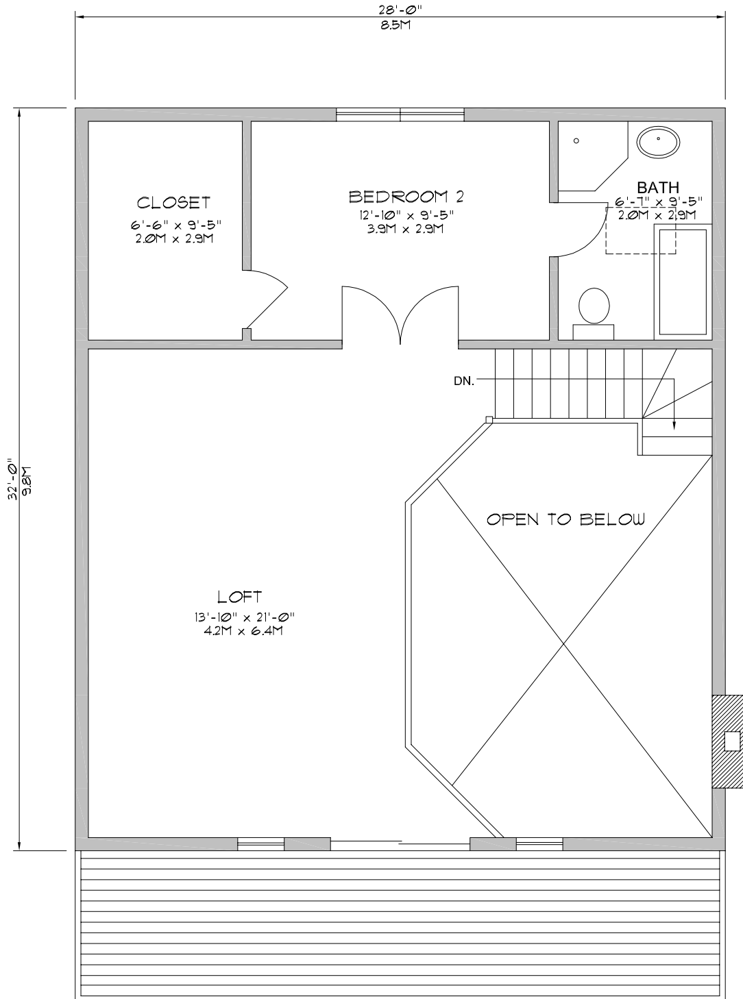
THE CHALET - UPPER FLOOR PLAN
