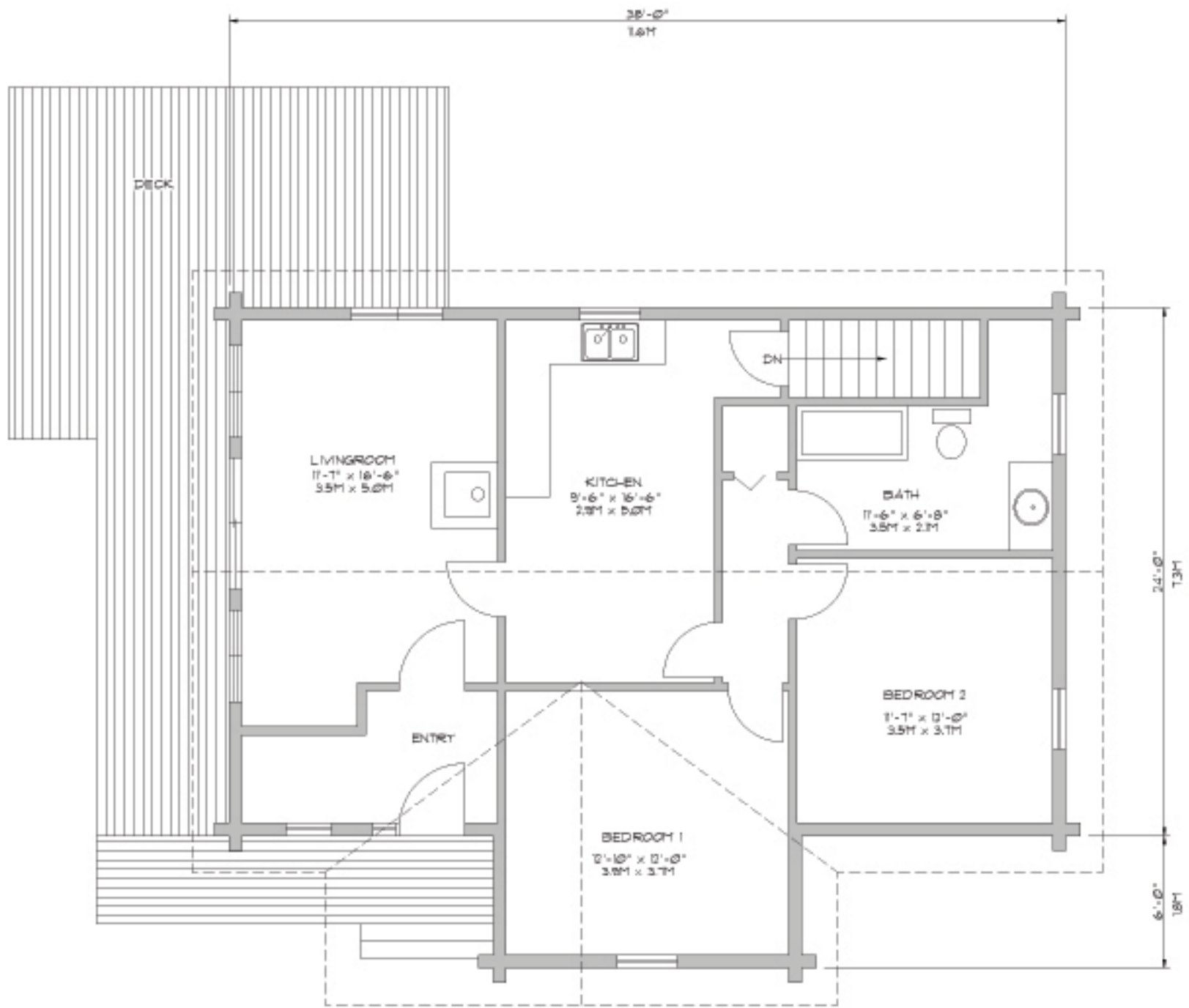
THE LAKE COTTAGE - FLOOR PLAN
